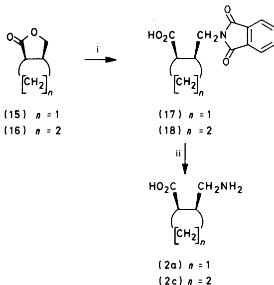
SCHEME 3 i, potassium phthalimide-DMF; ii, MeNH 2 -EtOH
