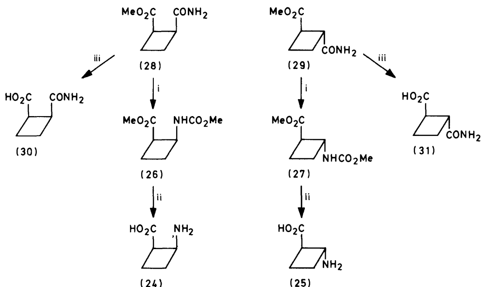
SCHEME 5 i, Pb(OAc) 4 -MeOH-PhMe; ii, (a) NaOH-aq. EtOH, (b) H + ; iii, NaOH-aq. EtOH
