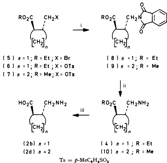
SCHEME 1 i, potassium phthalimide-dimethylformamide (DMF); ii, MeNH 2 -EtOH; iii, NaOH-aq. EtOH
