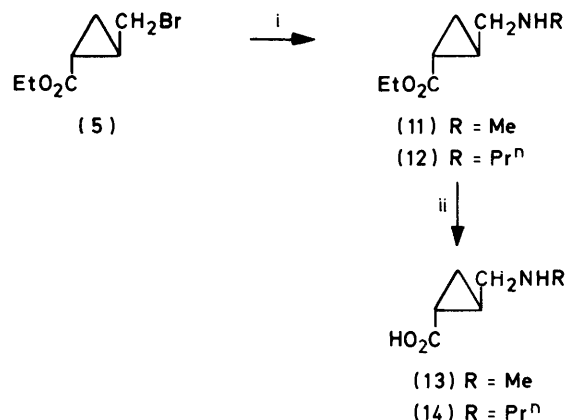
SCHEME 2 i, RNH 2 -PhMe or EtOH; ii, NaOH-aq. EtOH
