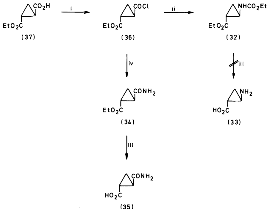
SCHEME 6 i, SOCl 2 ; ii, (a) NaN 3 -Me 2 CO-H 2 O, (b) heat, (c) EtOH; iii, NaOH-aq. EtOH; iv, NH 3 -PhMe
